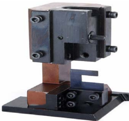
Radial Terminal Mold
